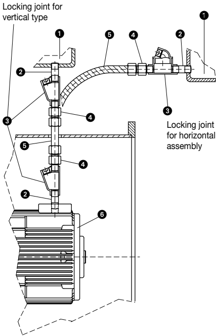
Fig. 4 - Cable exit with "Conduit" for Gas and Dust
