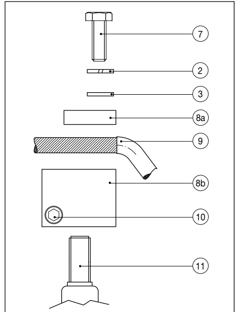
Figure 3 - Connection sequence 280÷315 (Cast iron frame)
