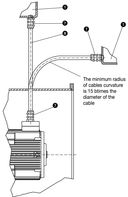
Fig. 6 - Cable exit with cable glands for Gas and Dust
